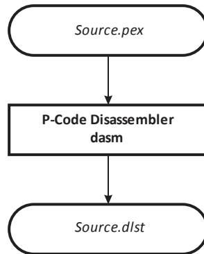
Figure 1. P-Code Disassembler
