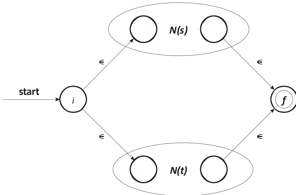
Figure 3. NFA for N(s|t)
