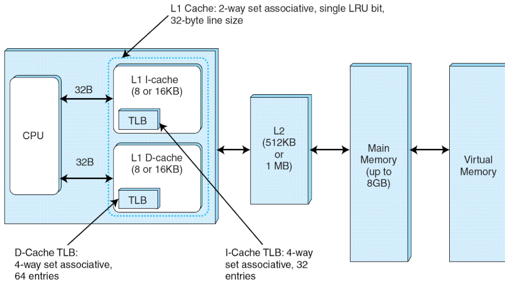
Figure 6.29 Pentium Memory Hierarchy
