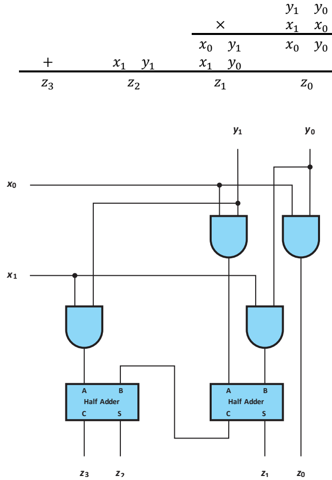
FIGURE 3.27 A simple Two-Bit Multiplier
