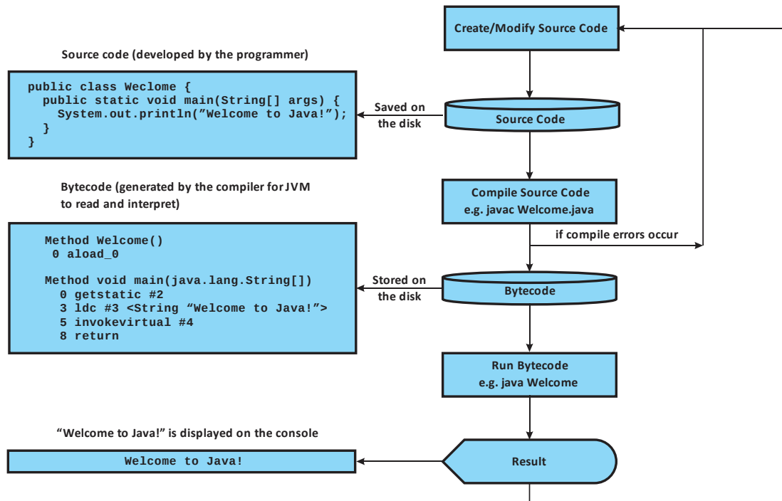
Figure 1.6 The Java program-development process consists of repeatedly creating/modifying source code, compiling, and executing programs
