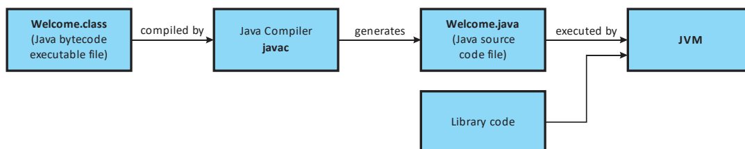
Figure 1.8 (a) Java source code is translated into bytecode.
